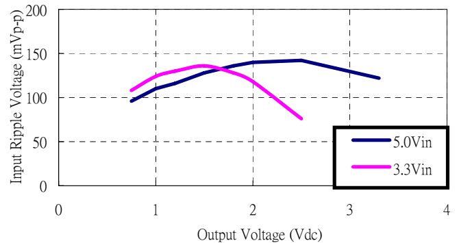
Figure 33: Input voltage ripple for various output models, IO = 10 A (CIN = 4x100 \mu F tantalum // 2x47 \mu F ceramic)
